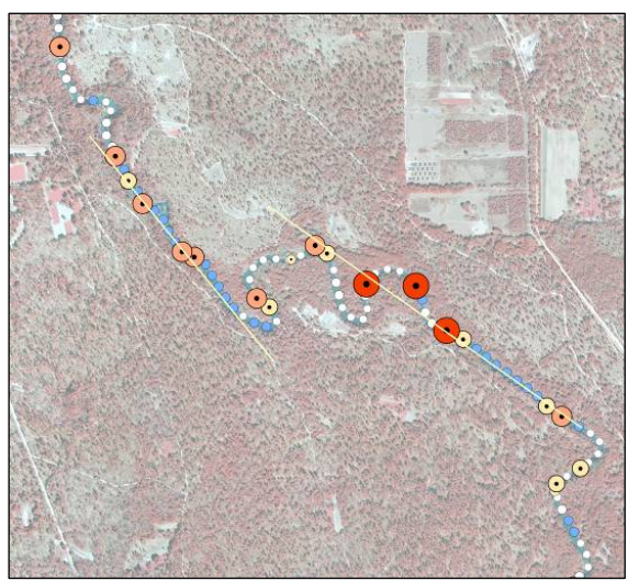
Figure 3. Comparison of calcium concentration and ^{18}\text{O}/^{16}\text{O} values in groundwater, precipitation and stream samples collected within the
