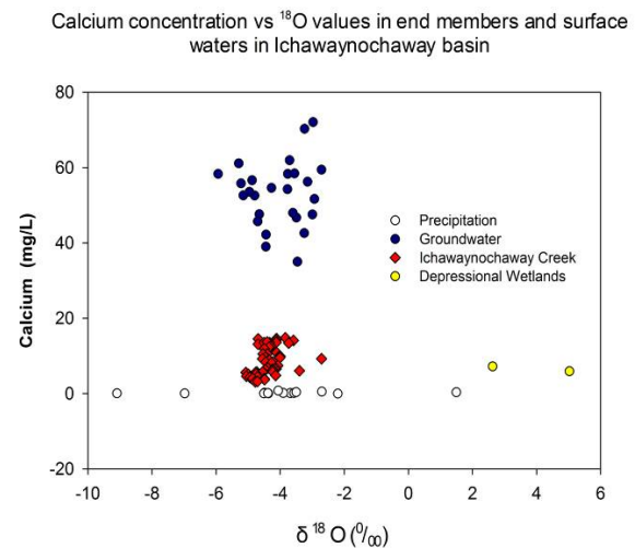
Figure 3. Comparison of calcium concentration and ^{18}\text{O}/^{16}\text{O} values in groundwater, precipitation and stream samples collected within the
